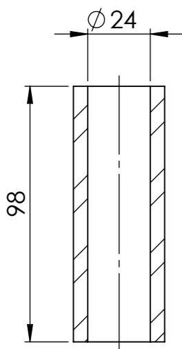
OUTPUT SHAFT
