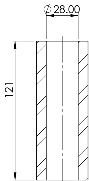
OUTPUT SHAFT
